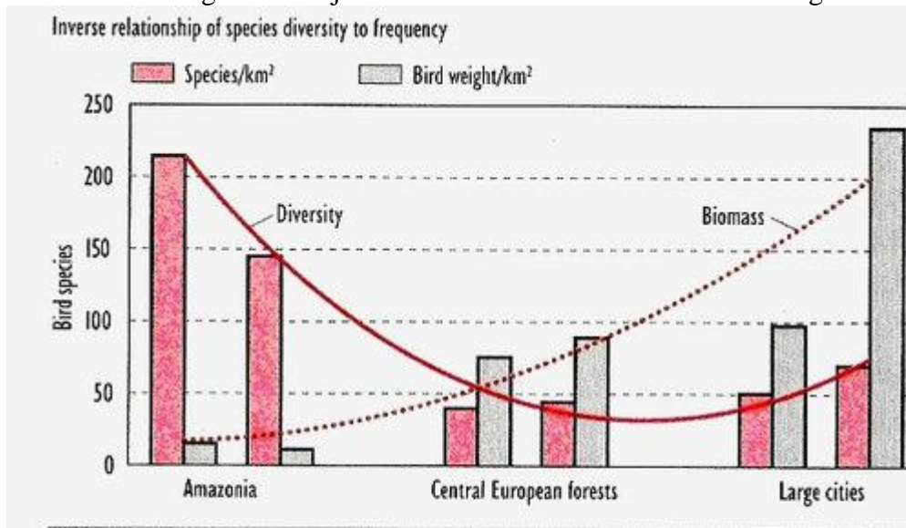
Figure 4 While Amazonia, the earth's most species-rich tropical forest, is home to many different bird species, the frequency of most of these is low. Central European forests, like other forests at climatically temperate latitudes, have considerably fewer species, but the birds occur at much higher frequency. The greatest frequency, however, is found in large cities
